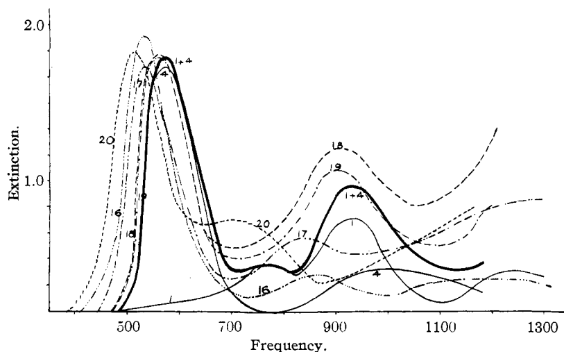
Fig. 3.—Absorption spectra of disazo dyes in a solvent containing 40 parts of 95% ethyl alcohol to 60 parts of concd. hydrochloric acid: dye 1, o -phenylazo- p -cresol; dye 4, p -phenylazodimethylaniline; dyes 16 to 20 as indicated in Table I.
